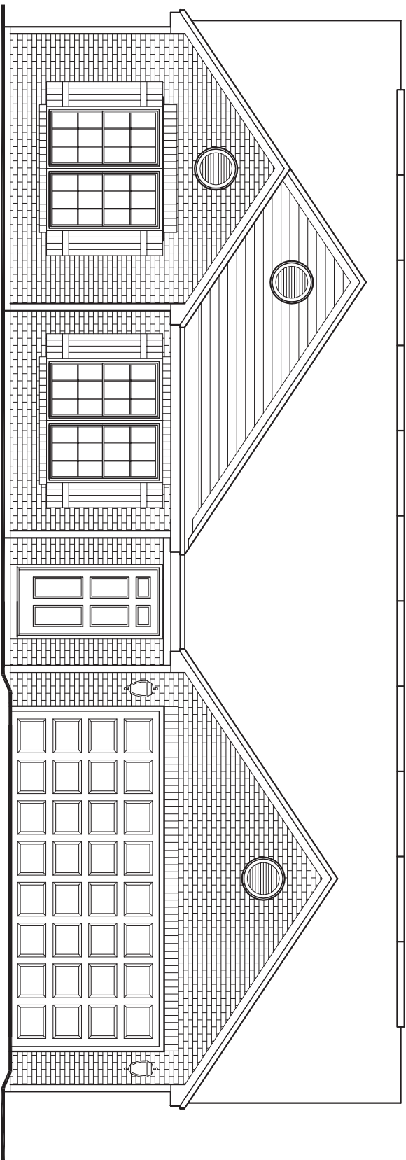
BRICK ACCENT ELEVATION
